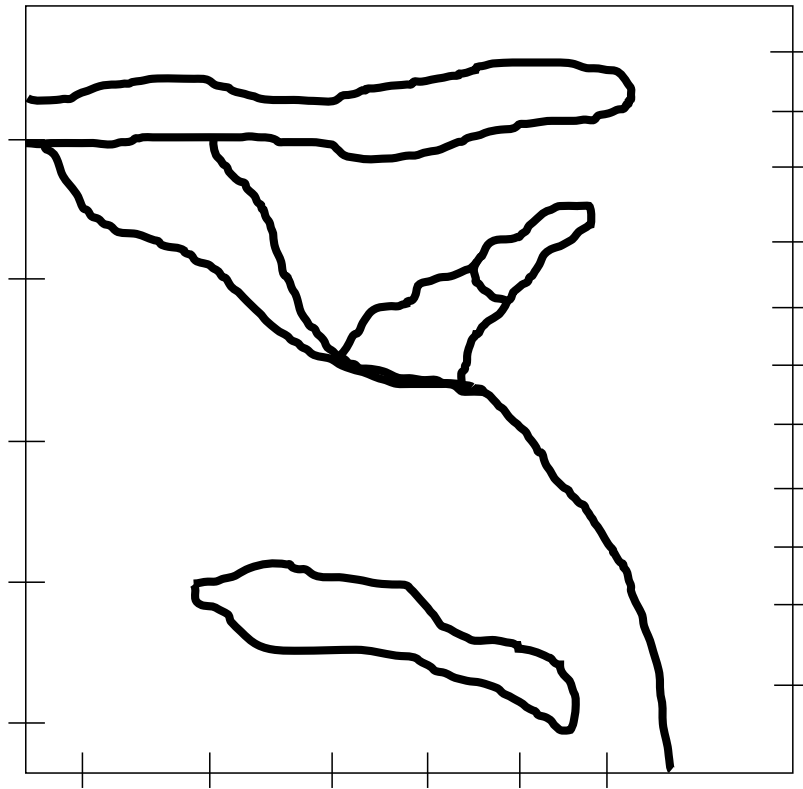
H _____ - R _____ Diagram
